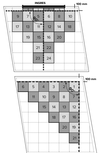
Posa Fortelock LIGHT, INDUSTRY, XL
